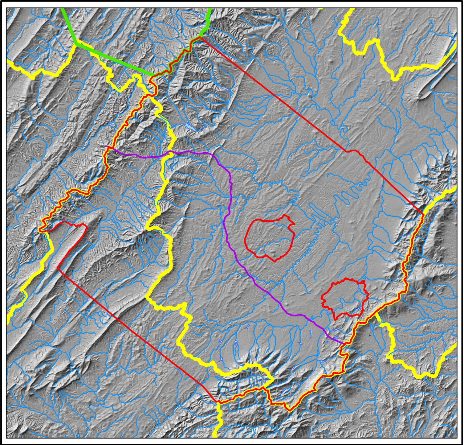
Figure 2: Regional Hydrography
